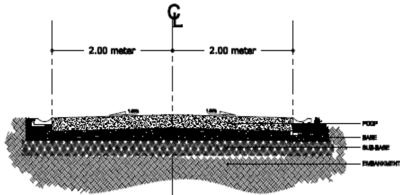
TYPICAL ROADWAY SECTION
