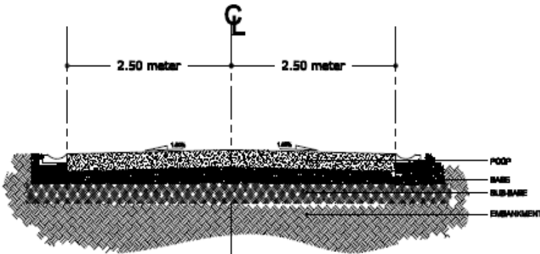
TYPICAL ROADWAY SECTION SCALE: NTS
